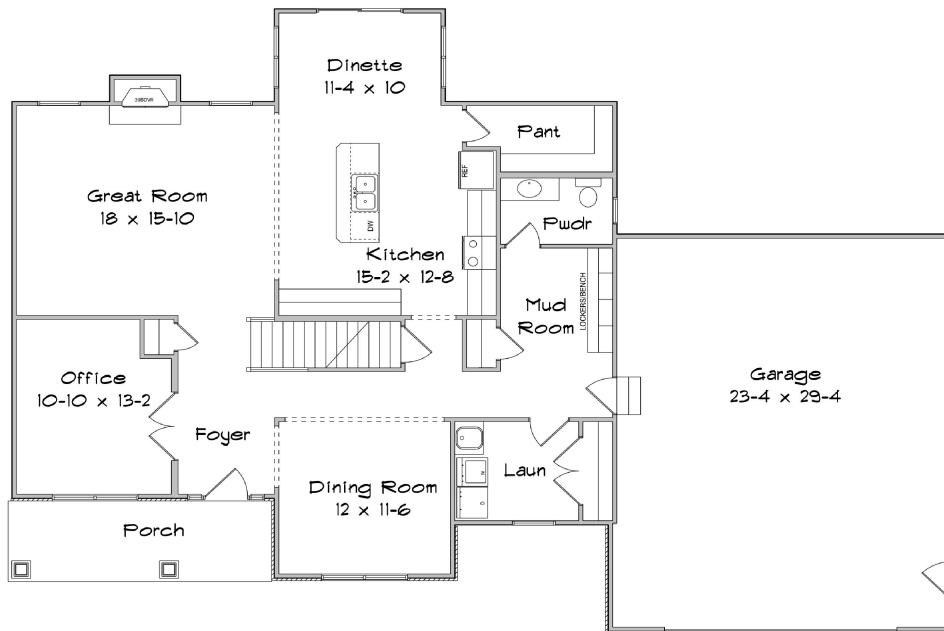
First Floor Plan 1450 Sq Ft
